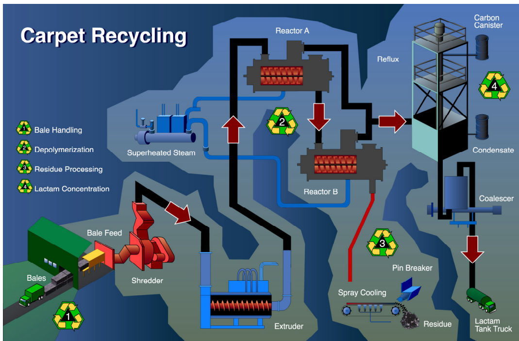
Abb. 21: Teppichrecycling Evergreen Nylon Recycling LLC 3 [18]
